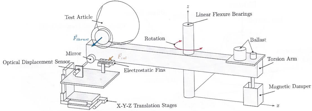
Fig. 2: Simplified Representation of Torsion Pendulum.
