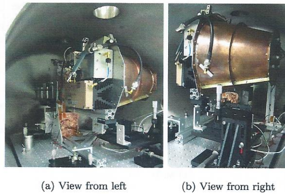
Fig. 14: Reverse Thrust Mounting Configuration.
