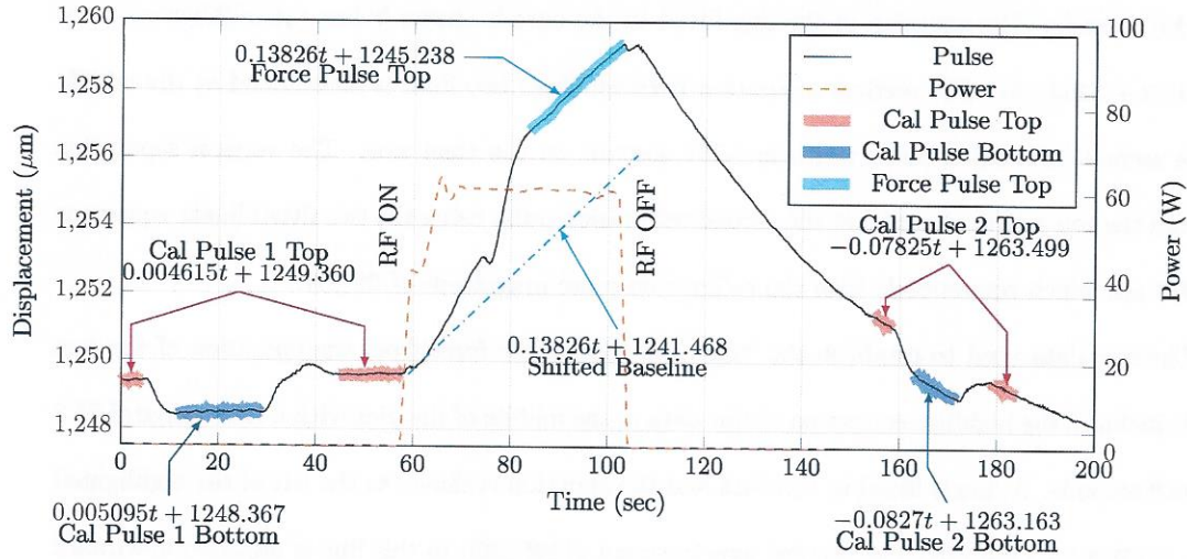
Fig. 8: Force Measurement Procedure Plot: The figure shows one of the 60W forward thrust runs with the data annotated to indicate the sections used to determine the calibration pulse characteristics, and the force pulse characteristics.
