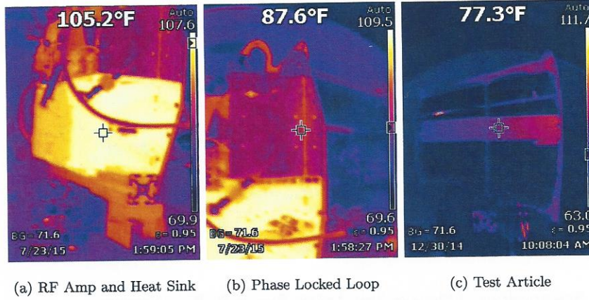
Fig. 6: IR Imagery of Test Article After Testing: Left pane shows RF Amp and heat sink; middle pane shows phase locked loop; right pane shows copper test article. Imagery was taken by a Fluke Ti100 Thermal Imager.
