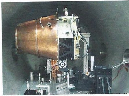
Fig. 11: Forward Thrust Mounting Configuration (heat sink is black finned item between test article and amplifier).
