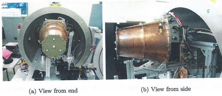
Fig. 17: Null Thrust Mounting Configuration.
